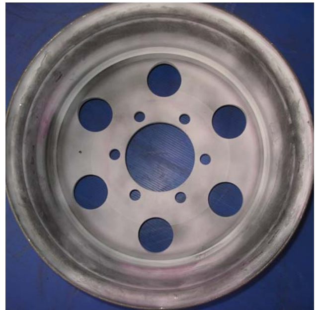
After 1 500 000 cycles radial fatigue no failure evident
